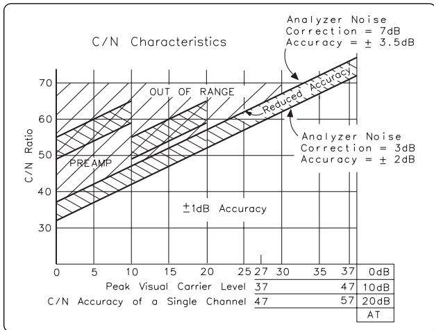
C/N accuracy (single channel) ± 1 dB accuracy
